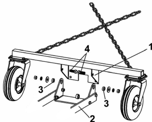
Install the subframe to the wheel support
