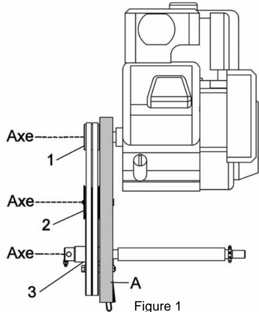
Figure 1 Back view of snowblower
