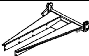
(088966) #700420 SUBFRAME EXTENSION KIT Used to install snowblower onto A.T.V
