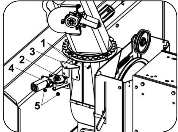
Motor installation
