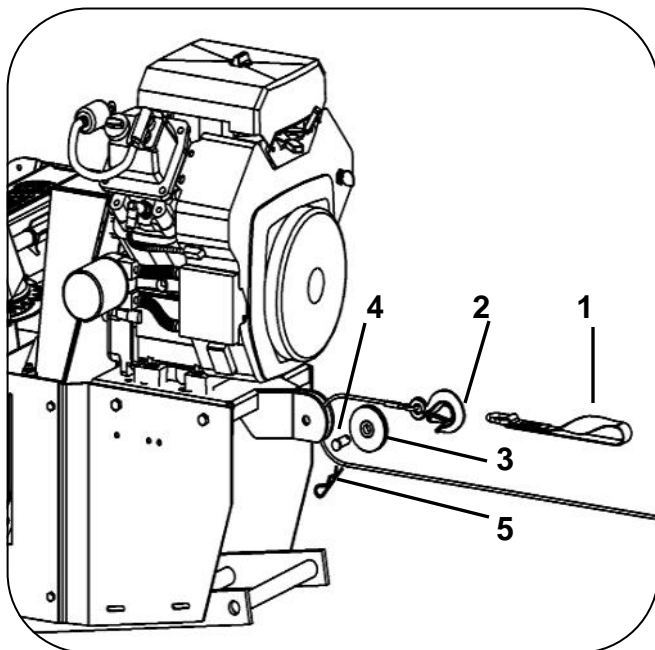
Lift system
