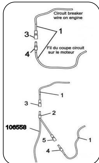
Connecting the engine circuit breaker wire
