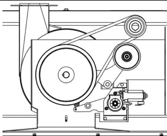
Figure 2 Side view of snowblower
