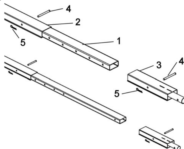
Adjust the length of the subframe
