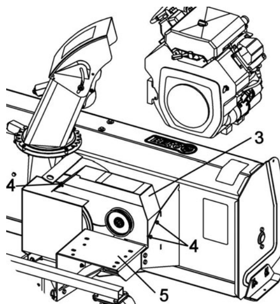
Install engine
