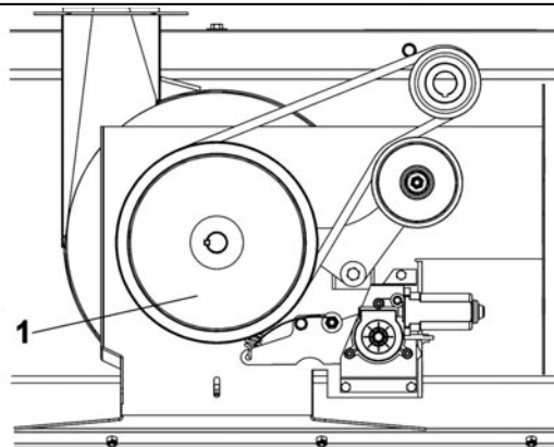
Figure 2 Side view of snowblower
