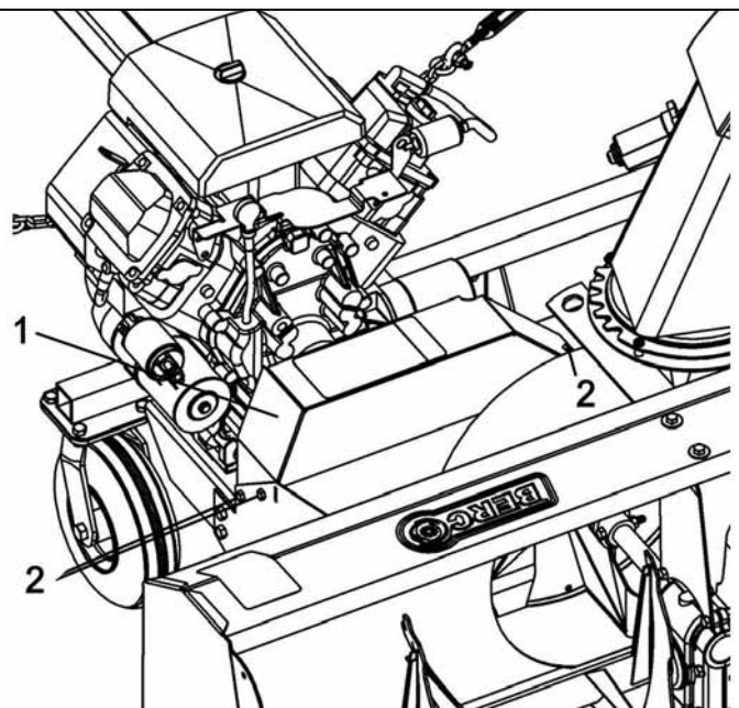
Install belt guard
