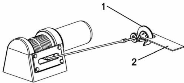
Install the winch cable
