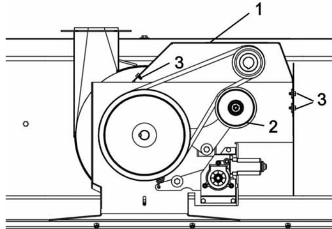
Belt replacement
