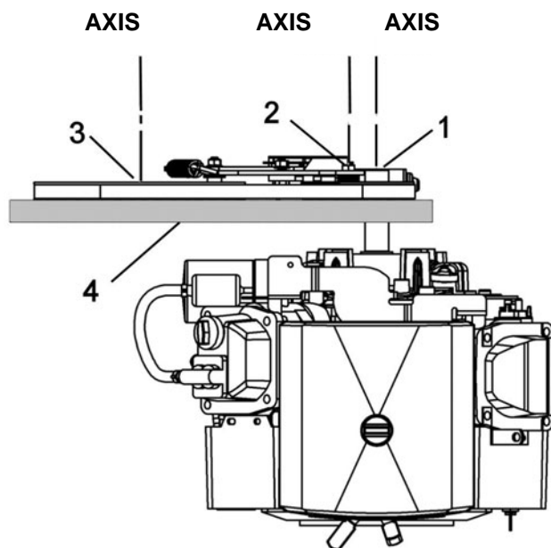
Figure 1 Top view of snowblower. All the pulleys are aligned and the engine is well installed.
