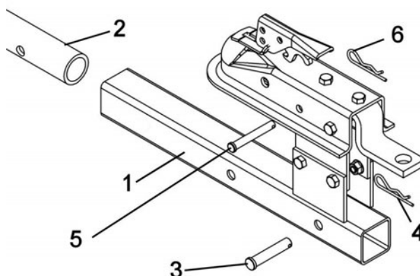
Secure the hitch support on the tow hitch ball
