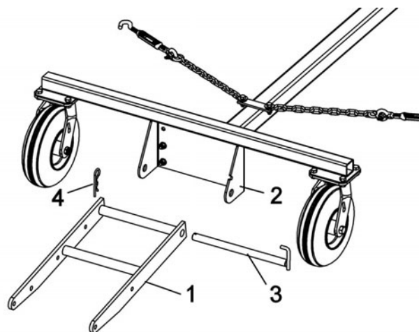
Install snowblower hitch
